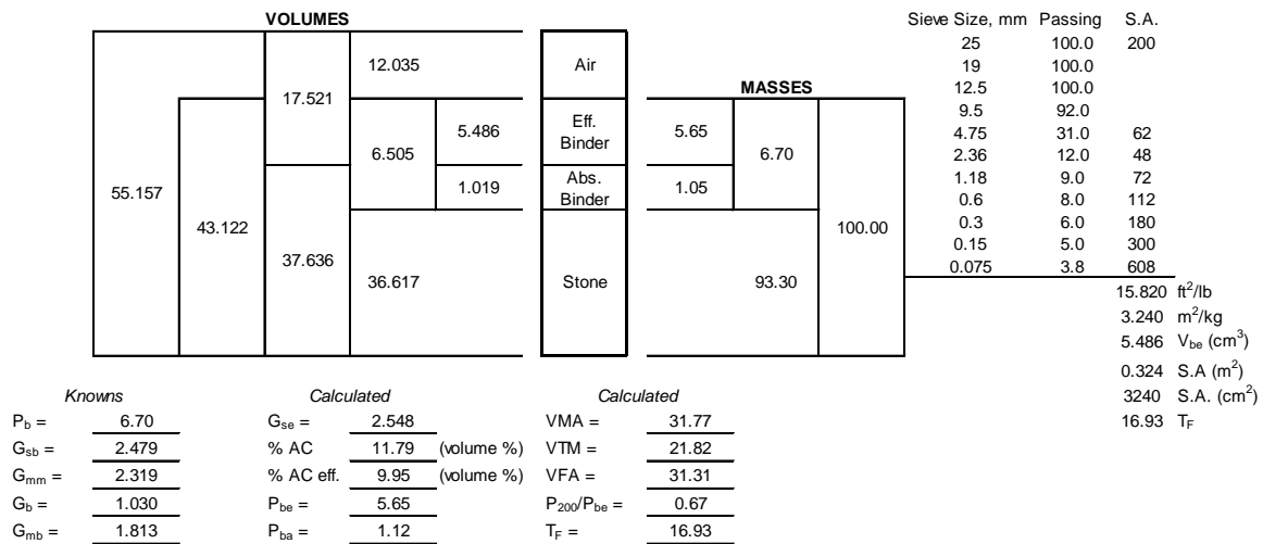
Figure 1.5 – Phase Diagram and Volumetric for Section S3 (Chert Gravel OGFC) of NCAT Test Track
