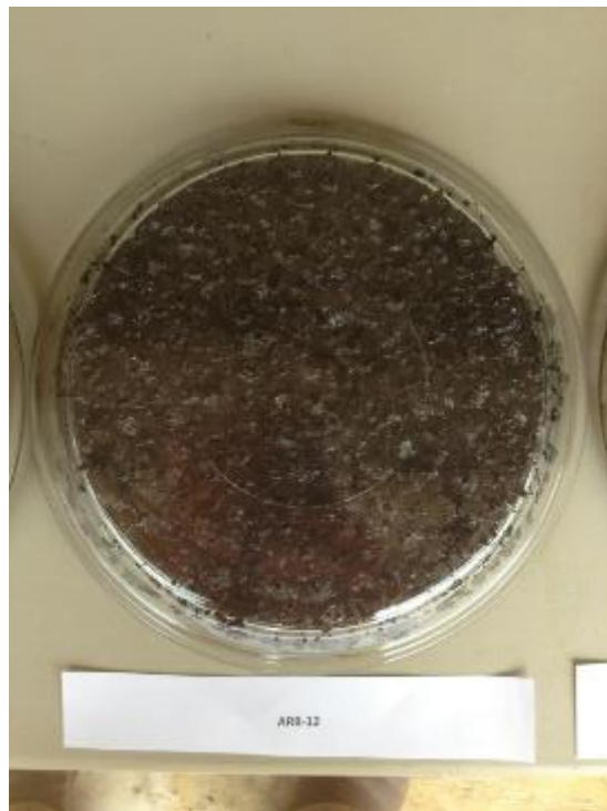
Figure 5.9 - Pie-Plate Test Results for Titan America FC-5 Mix at Optimum Asphalt Content; a) PG 67-22; b) PG 76-22; c) ARB-12
