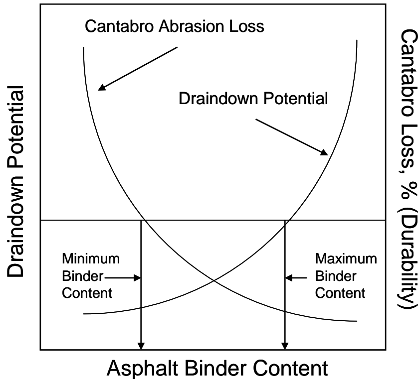
Figure 2.9 - Philosophy of Designing PFC Mixes
