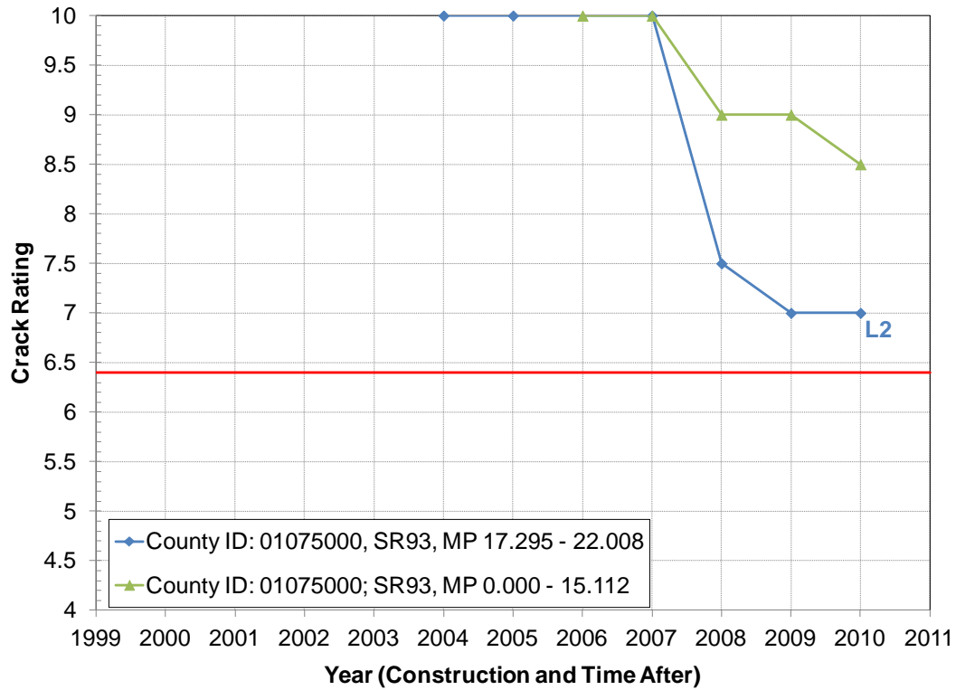
Figure 3.3 – FC-5 Cracking and Raveling Performance in District 1
