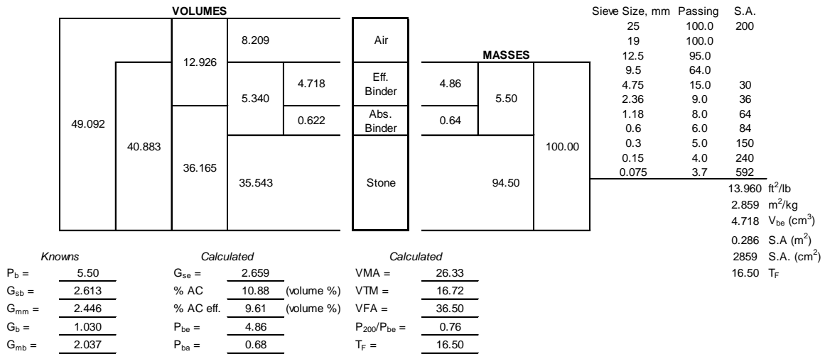
Figure 1.4 – Phase Diagram and Volumetrics of FC-5 Mixture at the NCAT Test Track Sections N1 and N2
