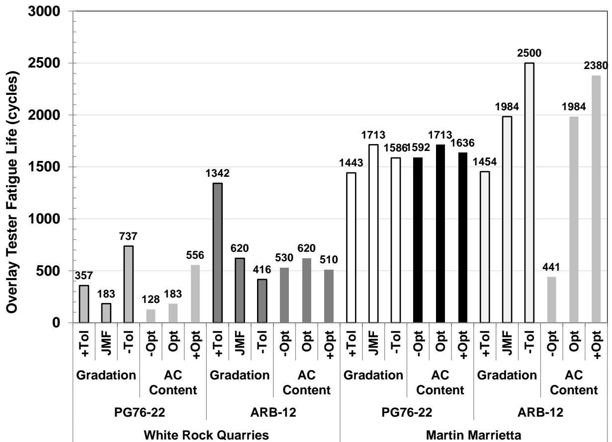
Figure 7.4 – Summary of Overlay Tester Results Due to Changes in Production Tolerances
