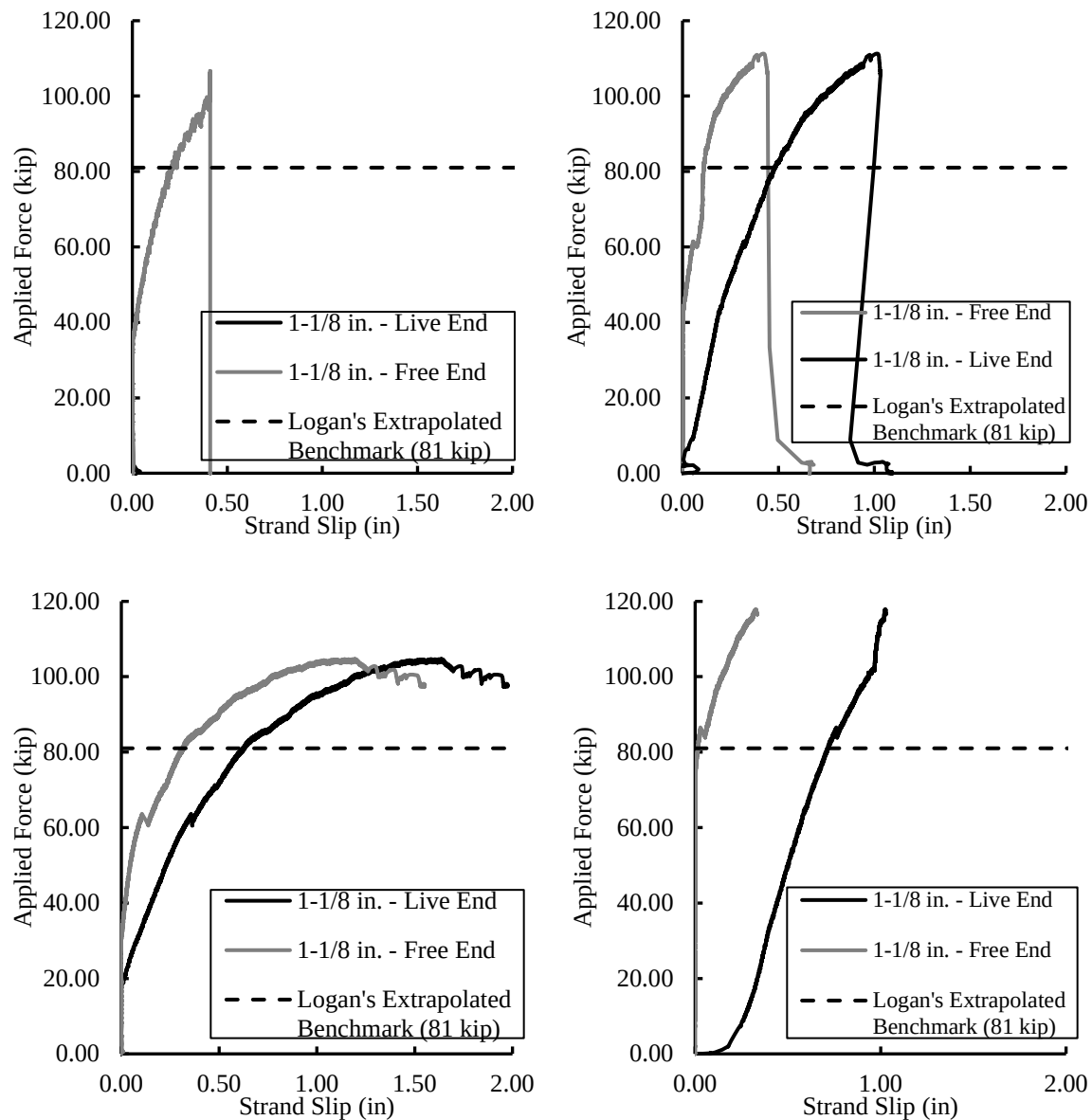
Figure A- 7 Slip versus load curves for 1-1/8 in. diameter strand (specimens 1-4 in 11980 psi concrete)
