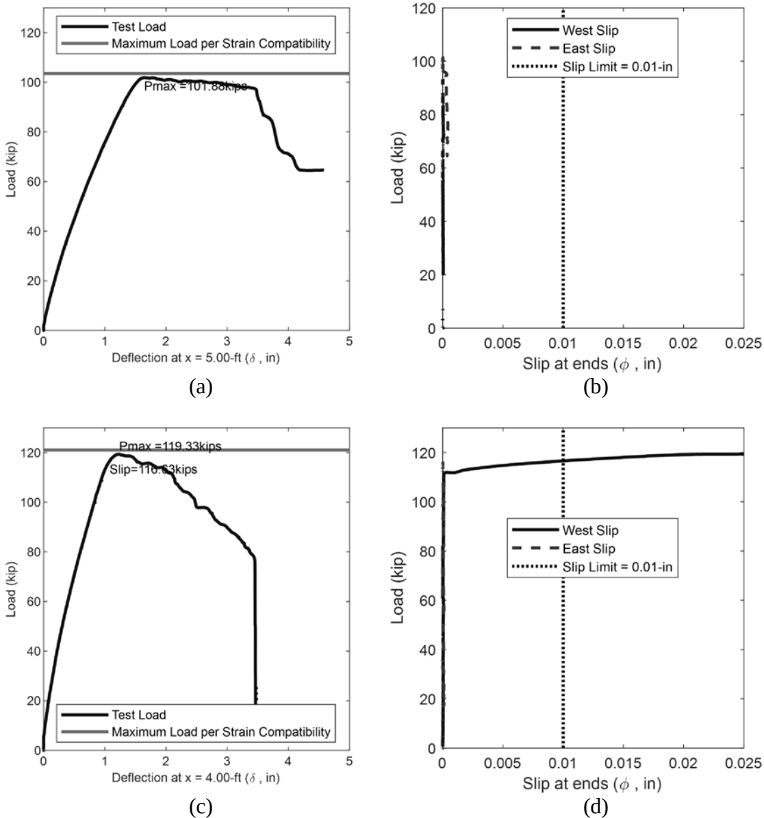
Figure 4-21 Load versus deflection curve for beam 7(a), load versus slip curve for beam 7 (b), Load versus deflection curve for beam 8 (c), and load versus slip curve for beam 8 (d)
