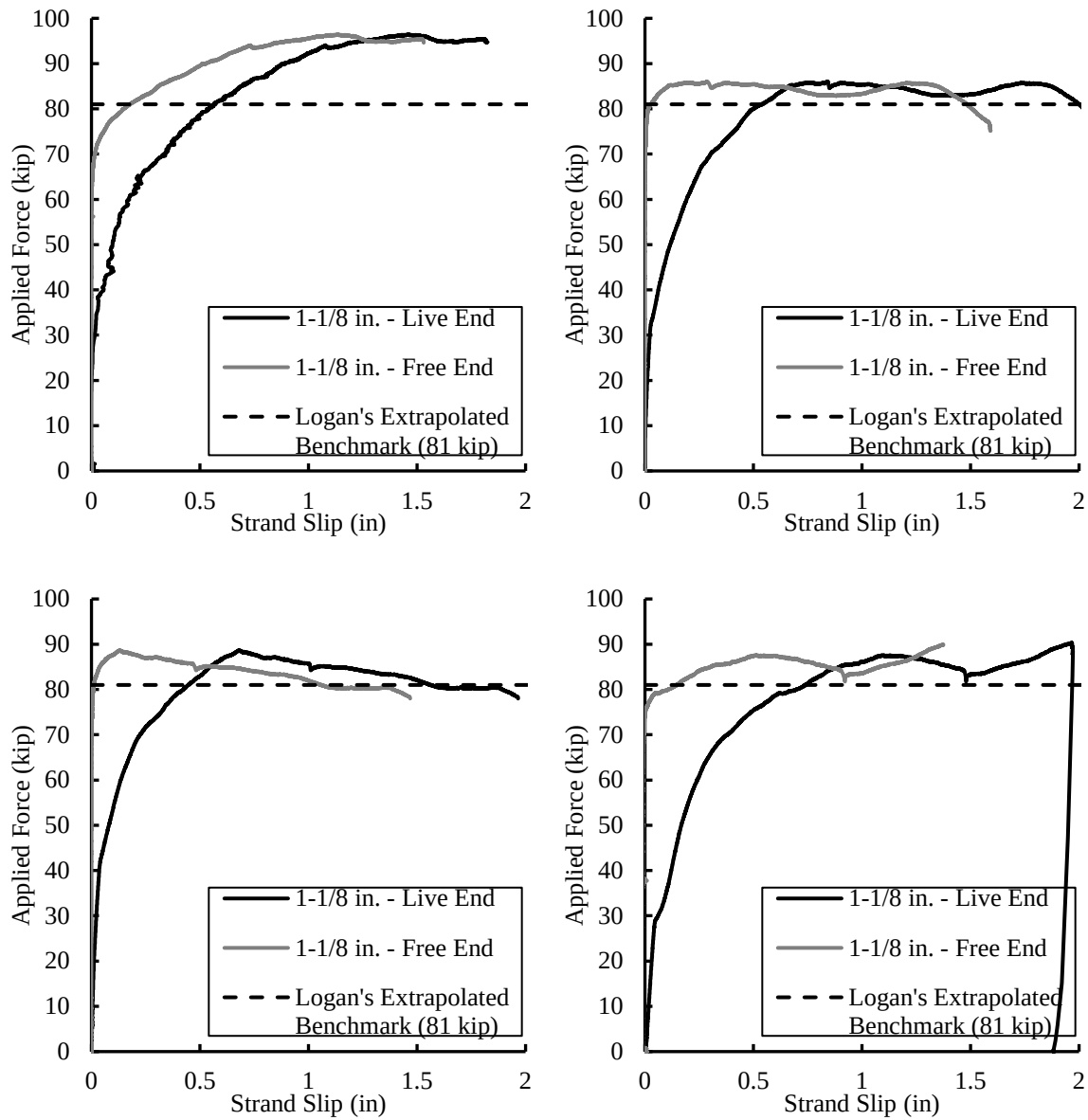
Figure A- 6 Slip versus load curves for 1-1/8 in. diameter strand (specimens 3-6 in 7303 psi concrete)
