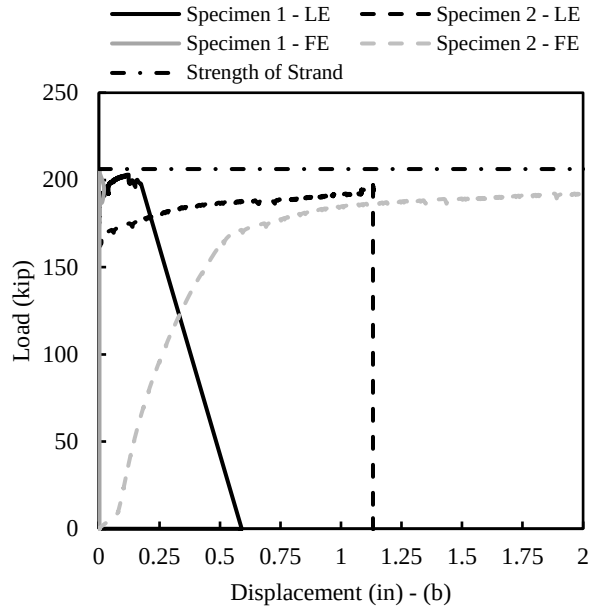
Figure 4-10 Pull out test results for 5-ft long specimens
