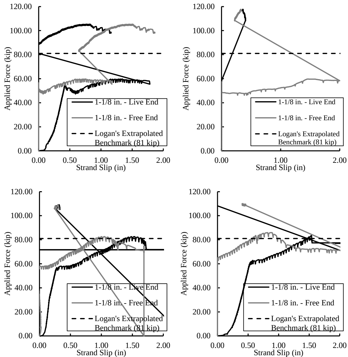
Figure A- 10 Slip versus load curves for rusted 1-1/8 in. diameter strand (specimens 3-6 in 6116 psi concrete)
