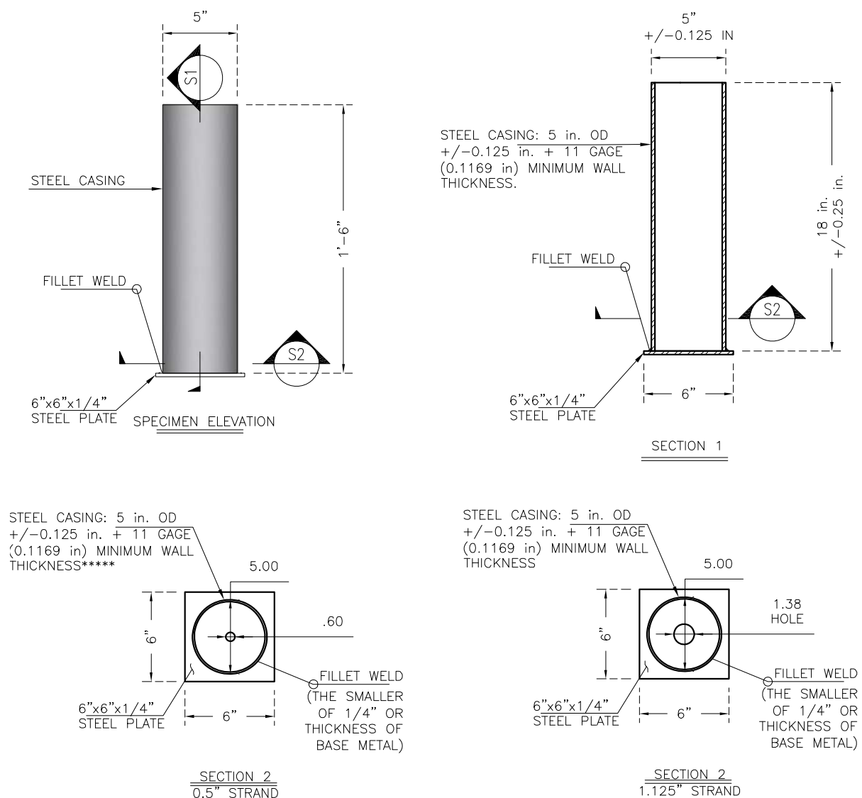
Figure 3-5 Illustration of the ASTM A1081 casing dimensions.
