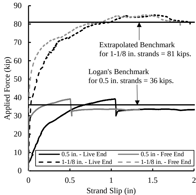
Figure 4-3 Example of LBPT results for 0.5 in. and 1-1/8 in. strands
