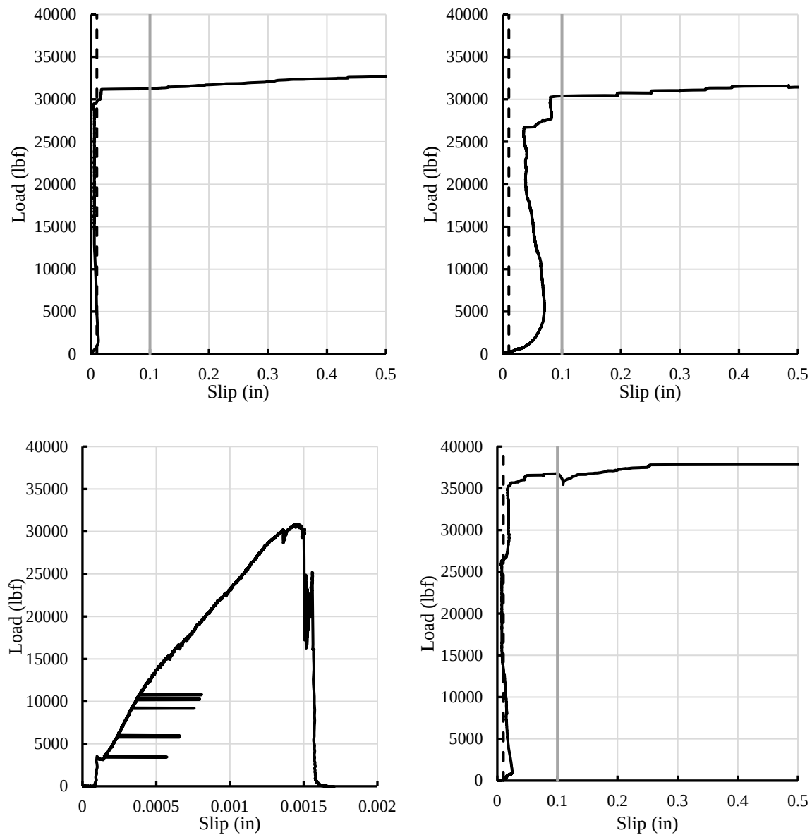
Figure A- 1 Slip versus load curves for 1-1/8 in. diameter strand specimens 1-4
