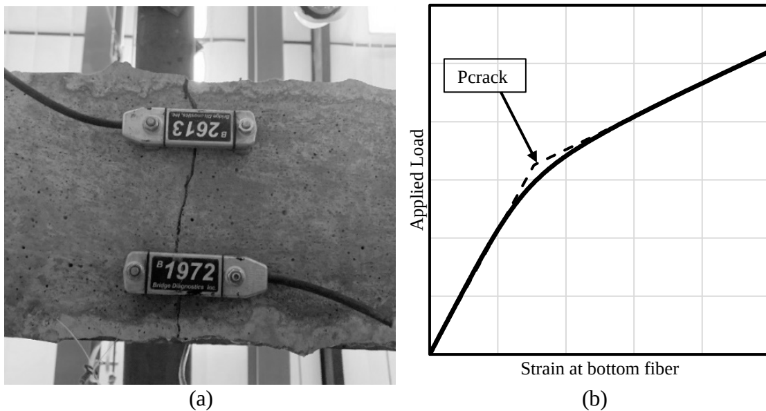
Figure 3-14 Illustration of the possible cracking load on a prestressed beam
