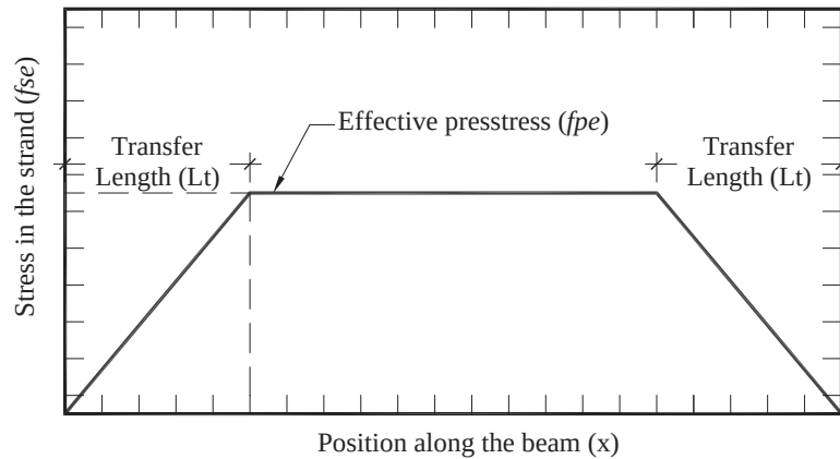
Figure 2-6 illustration of the transfer length
