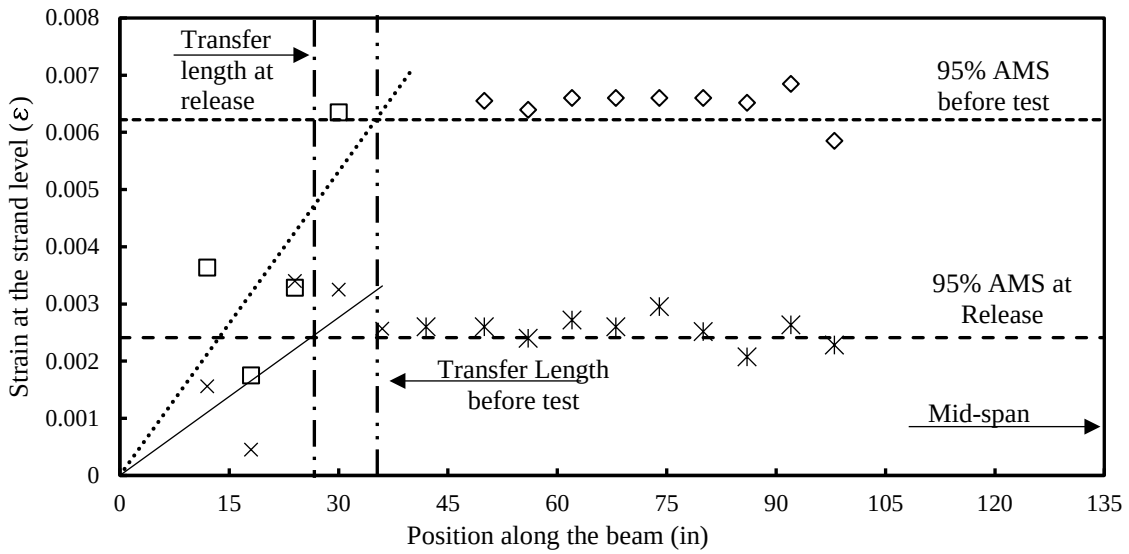
Figure A- 20 DEMEC readings of dead end of beam 4 side 2
