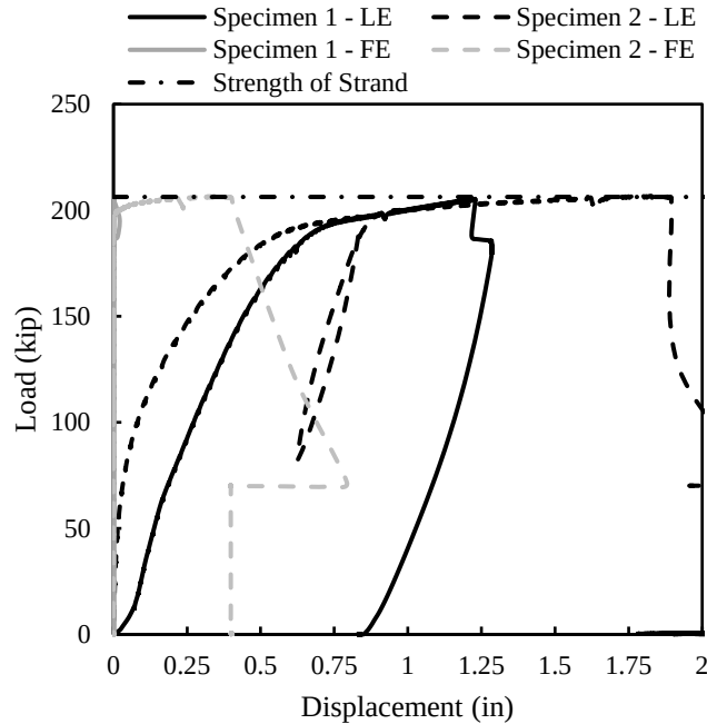
Figure 4-13 Pull out test results for 8-ft long specimens
