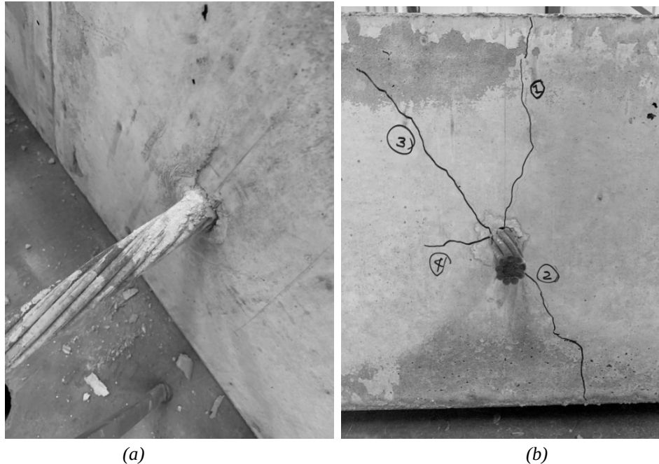
Figure 4-4 Rusted strand after the test (a), noticeable cracking on dead end (b)
