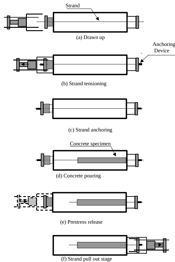
Figure 2-4 ECADA Test procedure
