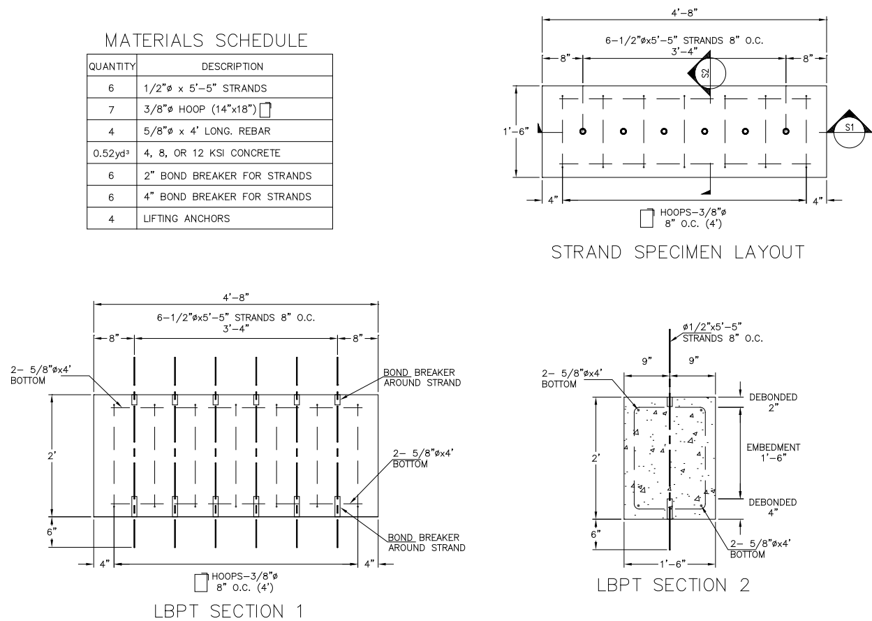
Figure 3-1 1/2 in. LBPT Specimen dimensions and strand layout
