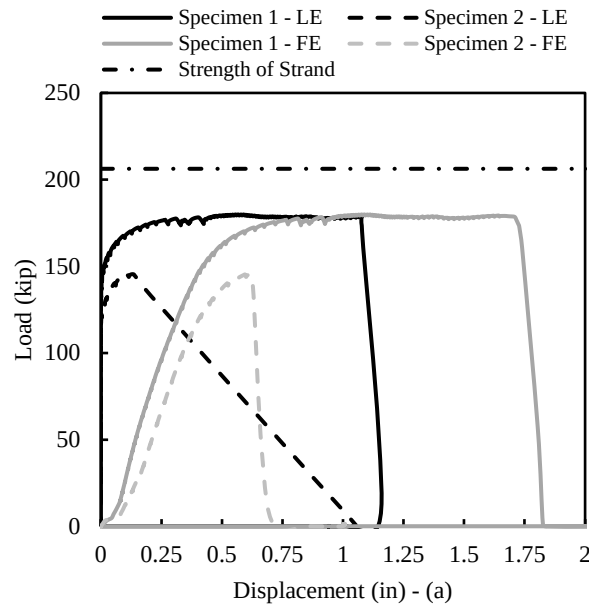
Figure 4-8 Pull out test results for 4 ft
