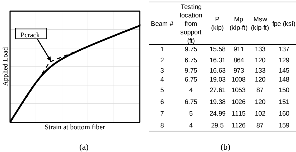
Figure 4-16 Surface strain gauges placed at the bottom fiber (a), effective prestress on the strand ( f_{pe} ) and calculations (b)
