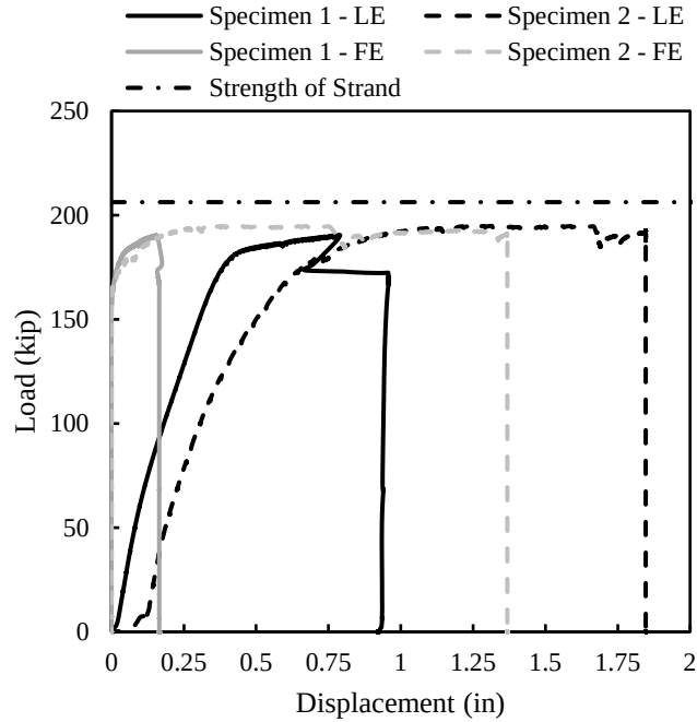
Figure 4-12 Pull out test results for 6-ft.
