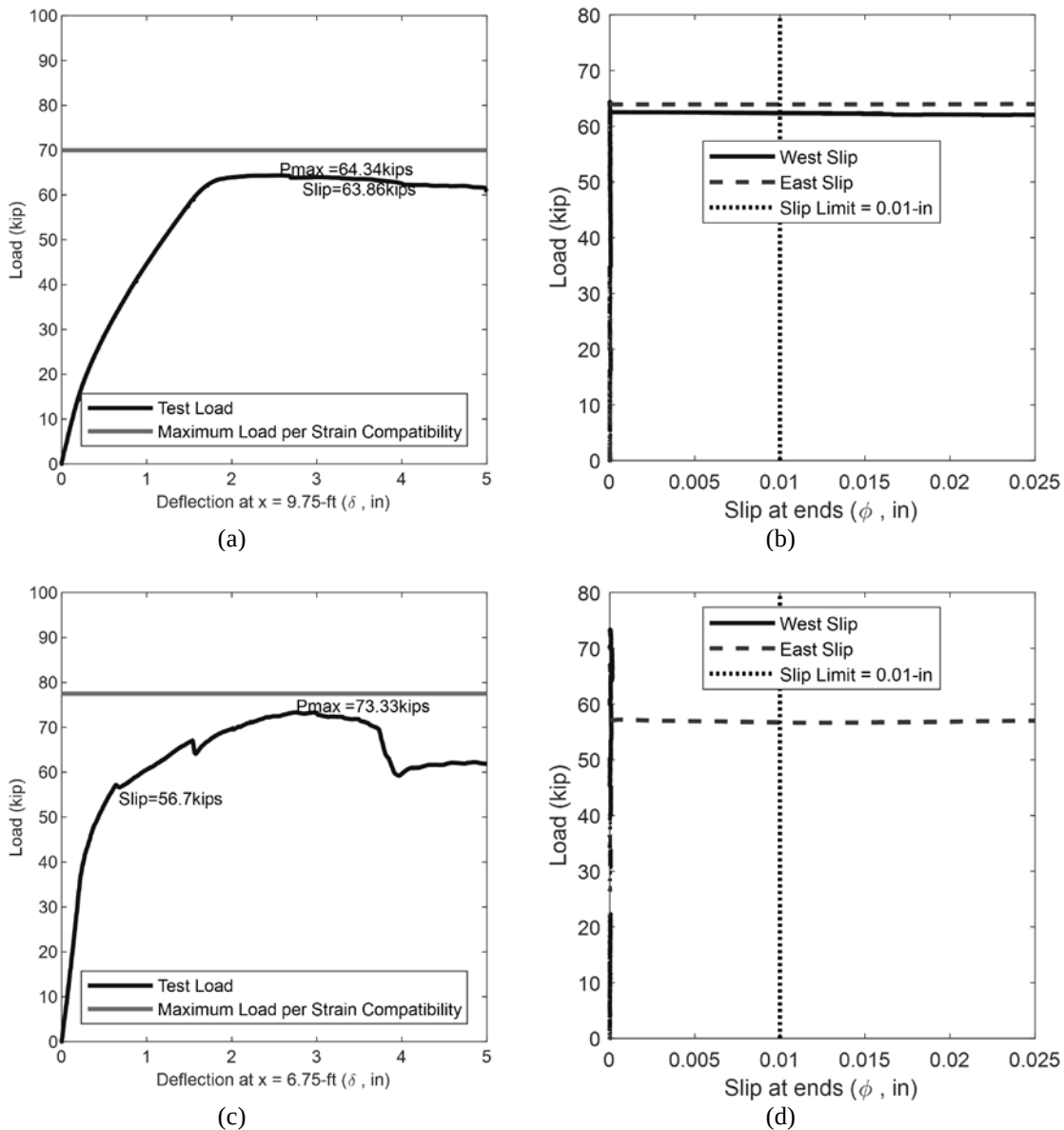
Figure 4-18 Load versus deflection curve for beam 1(a), load versus slip curve for beam 1 (b), Load versus deflection curve for beam 2 (c), and load versus slip curve for beam 2 (d)
