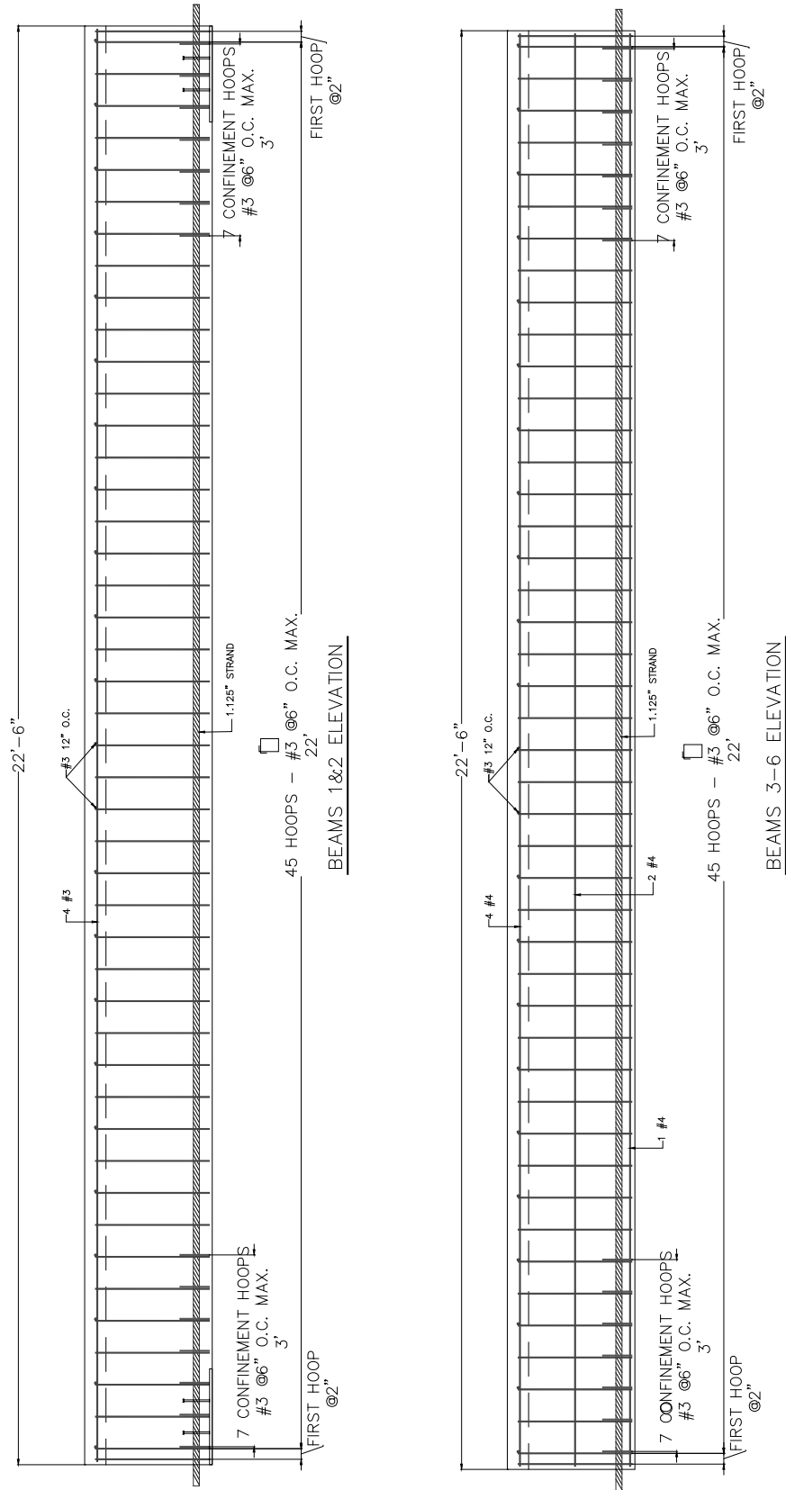
Figure 3-10 Elevation view of reinforcement for beams 1-8
