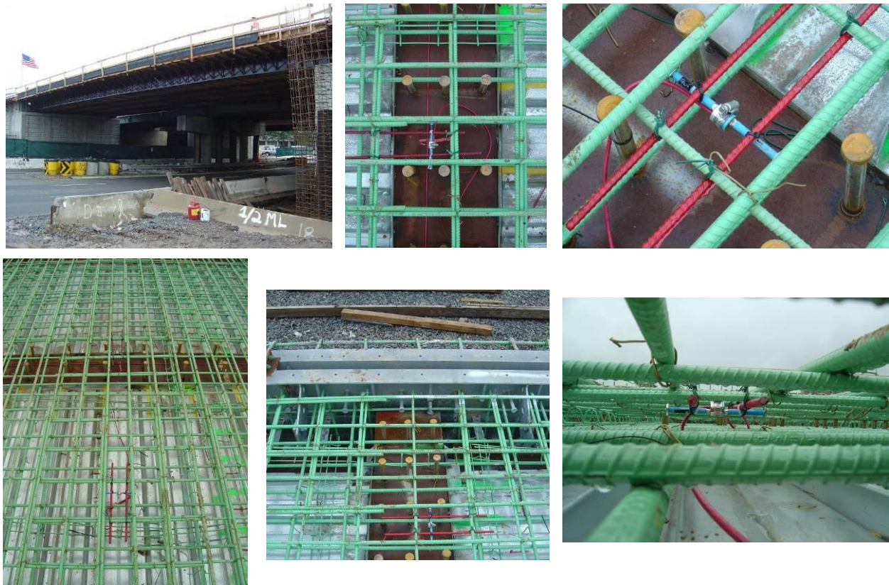
Figure 9. Vibrating wire strain gage installation
