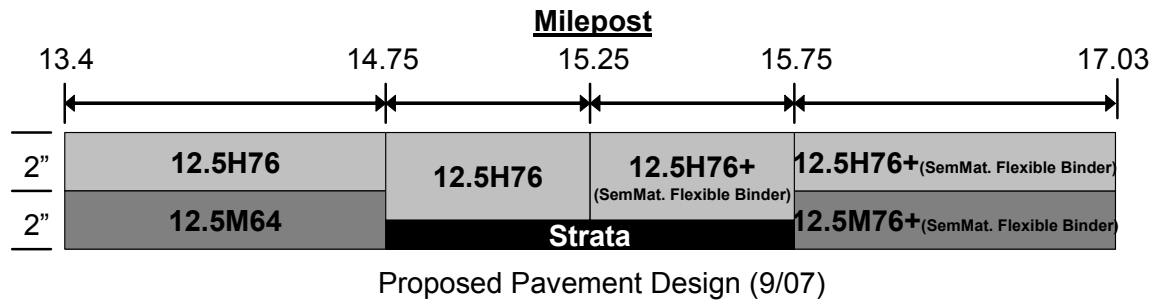
Figure 40 – Cross Section of Research Test Sections on Rt. 202S in New Jersey
