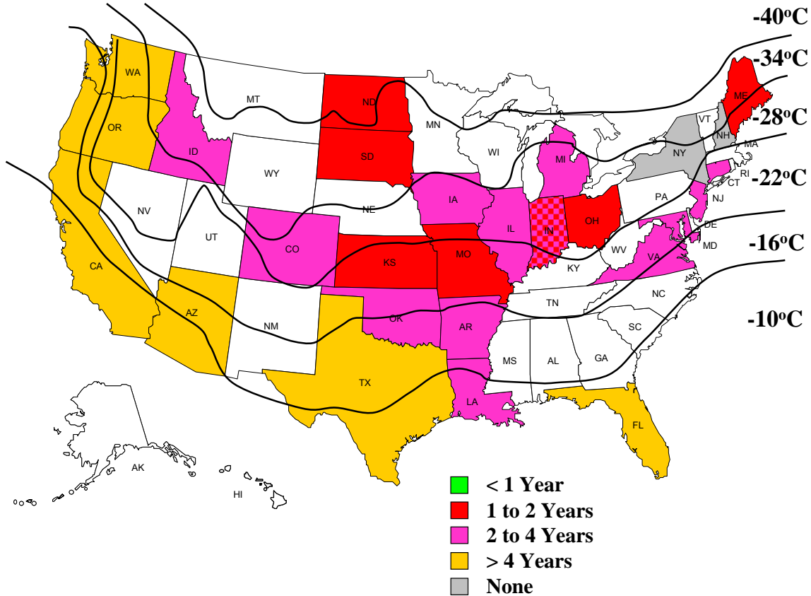
Figure 13(b) Time Until Reflective Cracking is Observed in HMA Overlay
