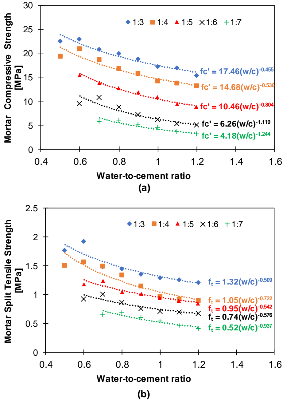
Figure 18: Cementitious material properties based on water-to-cement ratio and cement-to-sand ratio adopted by Singh et al. 45 ; (a) compressive strength (b) split tensile strength.
