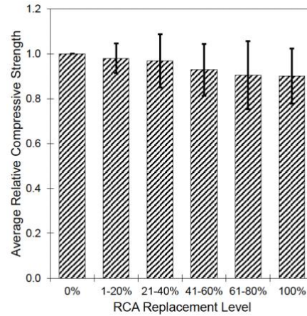
Figure 5: Average relative compressive strength of RAC systems compared to natural aggregate concrete systems
